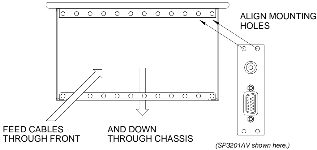
Diagram 7: Accessory Installation
