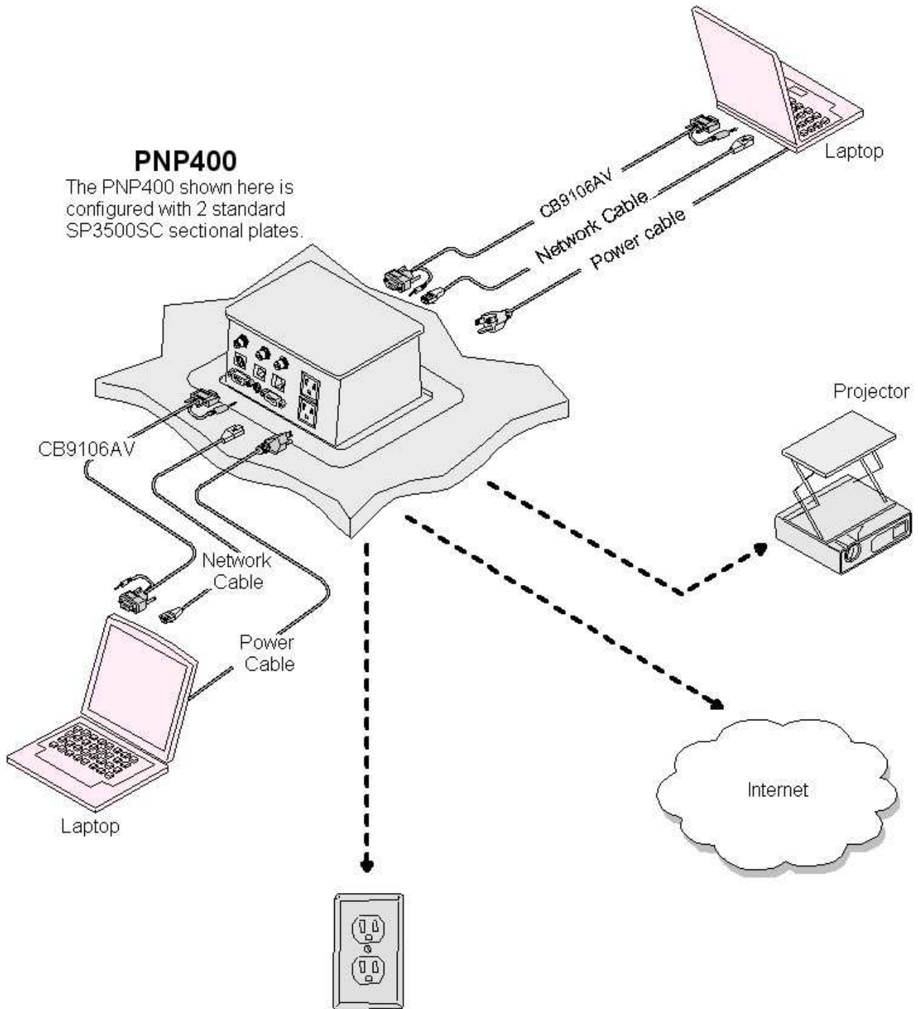
Diagram 1: Typical Setup
