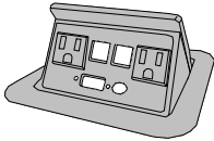
TNP320C CUSTOMIZABLE TABLE TOP WITH 2 POWER, 2 SNAP-IN CONNECTORS, 1 D-SUB, 1 AUDIO
