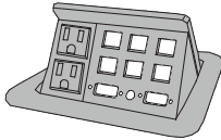
TNP528C 2 POWER, 6 SNAP-IN CONNECTORS, 2 D-SUBS, & 1 AUDIO
