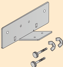
AG221-125 RT300-xxx MOUNTING HARDWARE FOR CNK221
