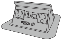
TNP328 (Black) HDMI, VGA, AUDIO, RJ45, 2 POWER
