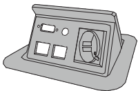
TNP421C GERMANY POWER WITH 2 SNAP-IN CONNECTORS, 1 D-SUB, & 1 AUDIO
